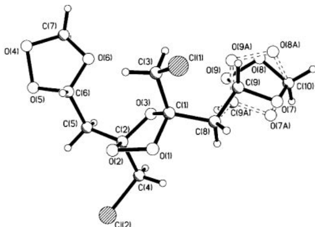
Figure 1. ORTEP diagram showing the X-ray structure of triozonide trans - 19a/b
